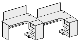
841PRx2/842x2/878x2/846x2/875x2 - 2800x1780x750(1150)
