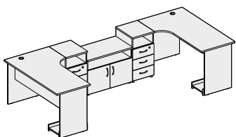
841PR/841L/842x2/878x2/813 - 3180x1400x750
