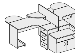
841.03L/841.03PR/842x2/878x2/813/819.60/109x2/874.01x2 - 2425x2050x750(1150)
