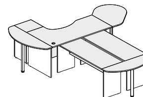
41L/20.01/42.04/66/109x2/13.01x2/63/147 - 2740x1310x750
