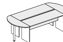
613.01x2/163x2/147x2 - 2800x2800x750(1120)
