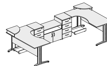
441L-Д/441PR-Д/142.04x2/178x2/174.01x2/105 - 2825x2800x750(1150)
