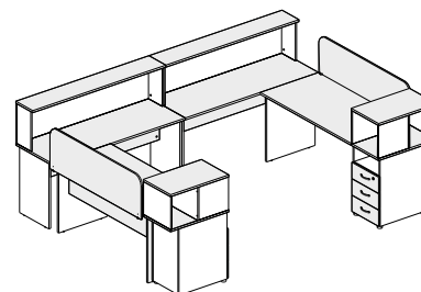
10x2/42x2/42.03x2/61x2/77x2/613.01x2/06.01x2 - 3200x2380x750(1120)
