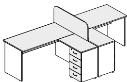
10x2/76x2/42.04x2/42.10x2 - 2825x1500x750(1140)
