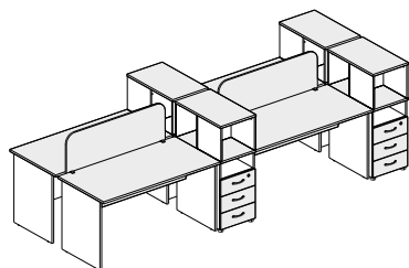
10x4/42x4/42.03x4/61x4/76x2 - 3580x1425x750(1120)
